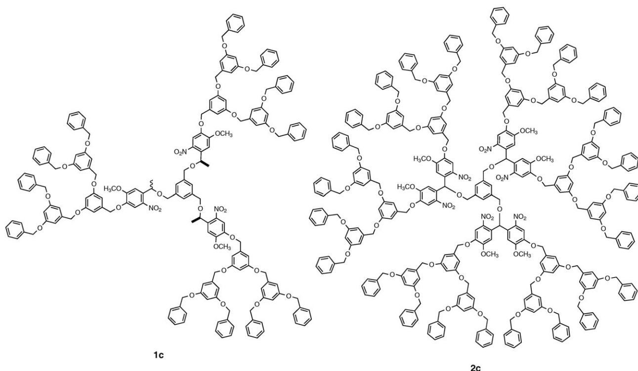
Chart 1 Structural formulas of second-generation dendrimer 1c and third-generation dendrimer 2c .
