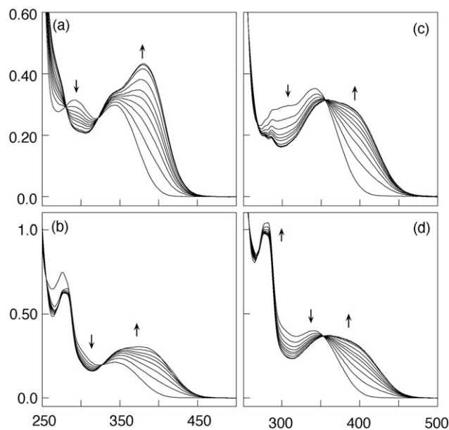
Fig. 1 UV-Vis spectra of the photolysis of 12 \mu\text{M} solutions ( \text{CHCl}_3 ) of (a) 1b , (b) 1c , (c) 2b and (d) 2c at t = 0, 2, 4, 6, 8, 10, 15, 25, 35, 45 min.
