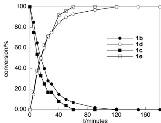
Fig. 3 Conversion of 1b to 1d and 1c to 1e as monitored by integration of the appropriate peaks in the ^1\text{H} NMR ( \text{CDCl}_3 ) spectra ( 1b : 3.97–3.91 ppm; 1d : sum of 4.09–4.06 and 3.90–3.87 ppm; 1c : 3.90–3.86 ppm; 1e : 4.05–4.02 ppm; TMS peak used for integration reference).
