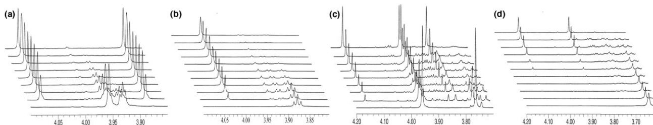
Fig. 2 ^1\text{H} NMR spectra of the photolysis of 5 mM solutions ( \text{CDCl}_3 ) of (a) 1b , (b) 1c , (c) 2b and (d) 2c at t = 0, 10, 20, 30, 40, 50, 60, 90, 120 ( 1c and 2c only), 150 ( 1c and 2c only), 180 min (proceeding upwards).
