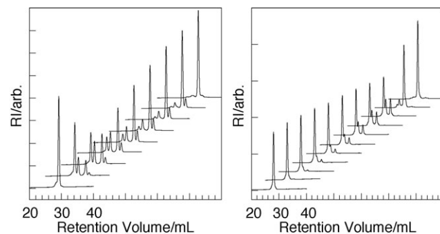
Fig. 4 GPC in \text{CH}_2\text{Cl}_2 of conversion of (left) 1c to 1e ( t = 0, 5, 10, 15, 20, 25, 30, 35, 170 min) and (right) 2c to 2e ( t = 0, 5, 10, 15, 20, 25, 30, 35, 40, 90, 140 min).
