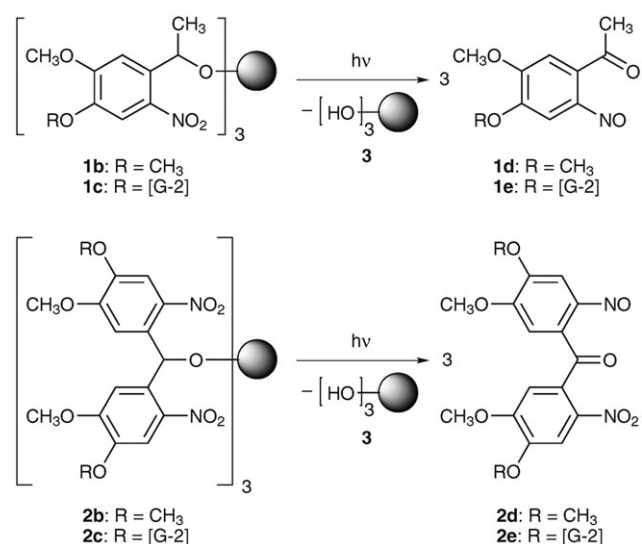
Scheme 2 Proposed degradation products from the photolysis of dendrimers 1b , 1c , 2b and 2c .
